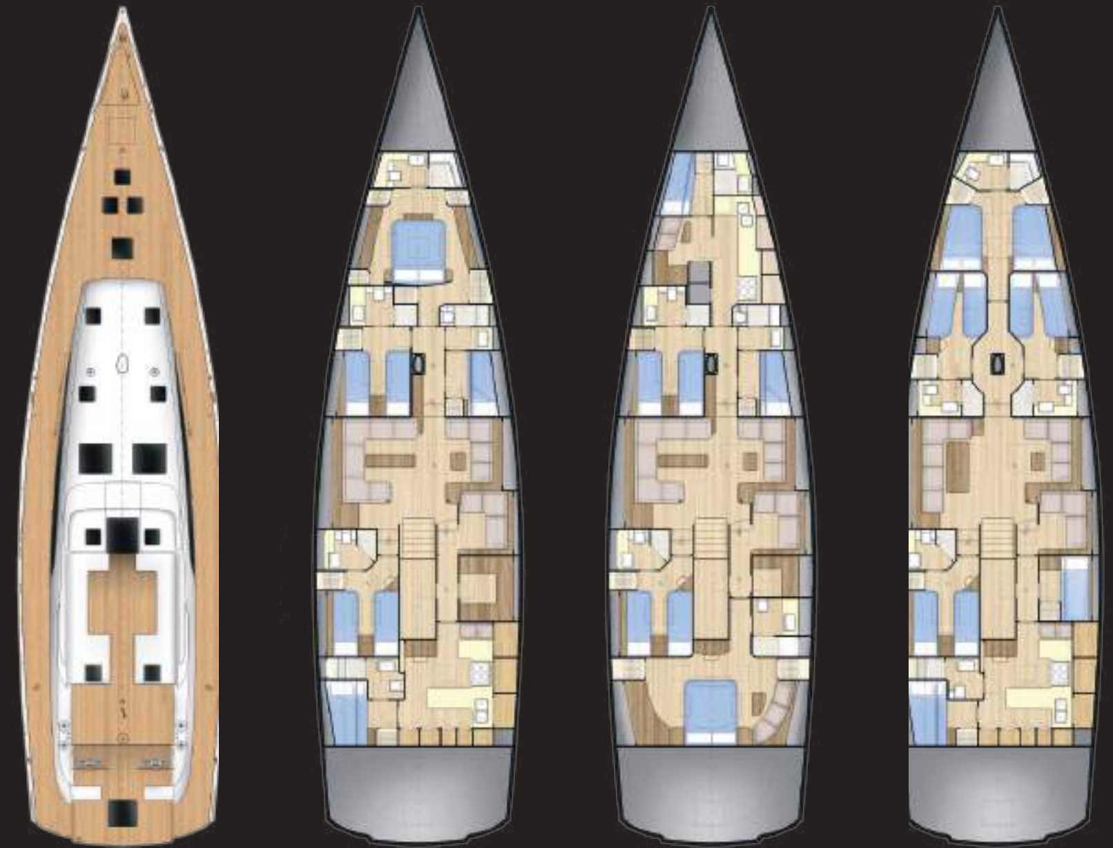
Preliminary layout
